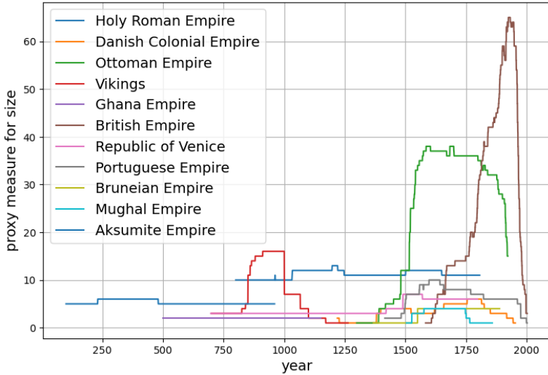
Figure 3. A few examples of the size proxy measure.
