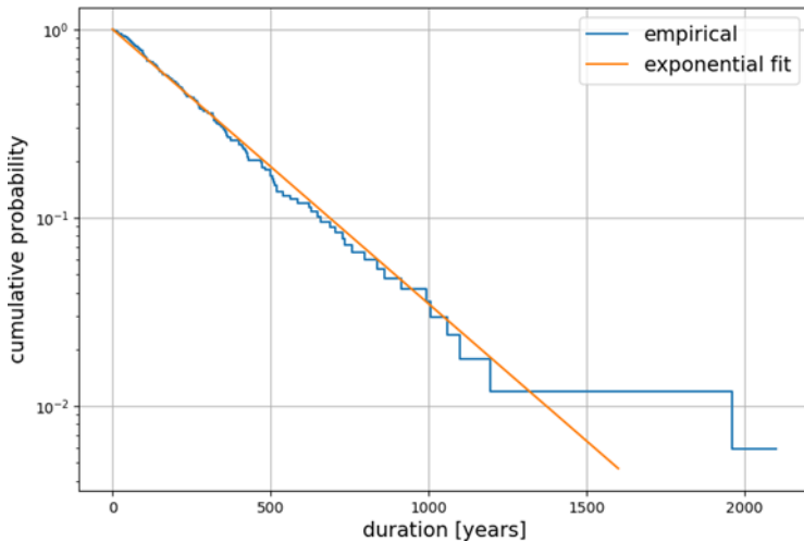
Figure 1. The cumulative distribution of empires' lifetime, along with the exponential fit. Note the log-scale on the y-axis.
