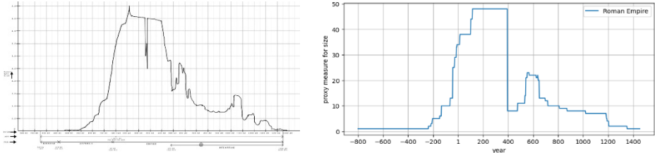
Figure 2. The example of Roman Empire: A comparison of our proxy measure of size (the number of countries included in an empire, right panel) with Taagepera’s chart (Taagepera 1979) (left). The similarity is strong and suggests that we can move forward with our experiment. Note that here we have aggregated Roman and Byzantine Empires, the purpose being the comparison with Taagepera’s plot.
