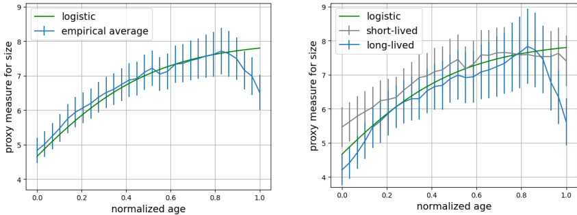
Figure 4. Left: the average size of empires is computed as a function of their normalized age; the logistic fit is also shown. Right: the average size is computed separately for short-lived and long-lived empires. See text for more explanations.
