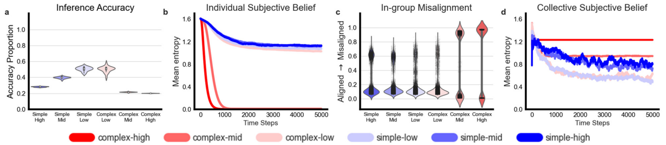
Figure 3: Simulation results across conditions (inference strategy*conformity bias strength): a ) Inference accuracy; b ) Mean entropy of individual subjective belief; c ) In-group misalignment; d ) Mean entropy of collective subjective belief.
