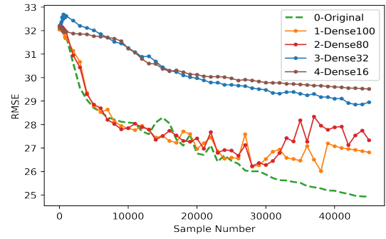
Figure 2: Test RMSEs over sample number for the BPMF with batch-10 uncertainty active strategy under different choices of input features dimensions.
