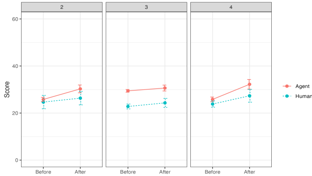
Figure 4: Average AIS before discussion → AGS after discussion
