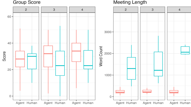
Figure 3: Left-panel: group score; Right-panel: meeting length in word count
