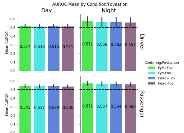
Figure 7: Mean and variance of AUROC among subjects for each task condition, driving condition, and foveation/centering condition.
