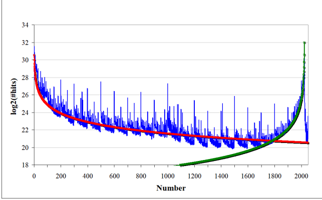
Figure 2: Querying numbers between 0 and 2050 on a search engine in logarithmic scale. The red curve is \log_2(\#hits(0)) - \log_2(N) , while the green curve is \log_2(\#hits(2023)) - 1.42 \log_2(\frac{2023-N}{0.35}) (the results are displayed for Yahoo, but we obtained superposable results with Bing and Google).
