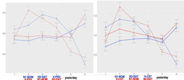
Figure 1: Results (SPR). Left: SP; Right: MC. X-axis: region; Y-axis: residual RT. Blue: VF; Red: VI. Solid line: NSK; dashed line: KHS. Error bars: 95% CI.
