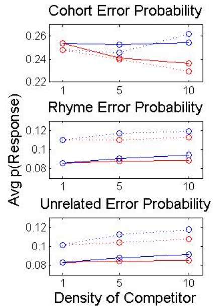
Figure 1: TRACE model predictions for effect of increasing rhyme density (red lines) or cohort density (blue lines) on probability of cohort errors (top panel), rhyme errors (middle panel), and unrelated errors (bottom panel). Solid lines show results of no-noise simulations, dotted lines show with-noise simulations. Note that the vertical axis scale differs in the top panel because cohort activations are substantially higher than rhyme and unrelated activations.
