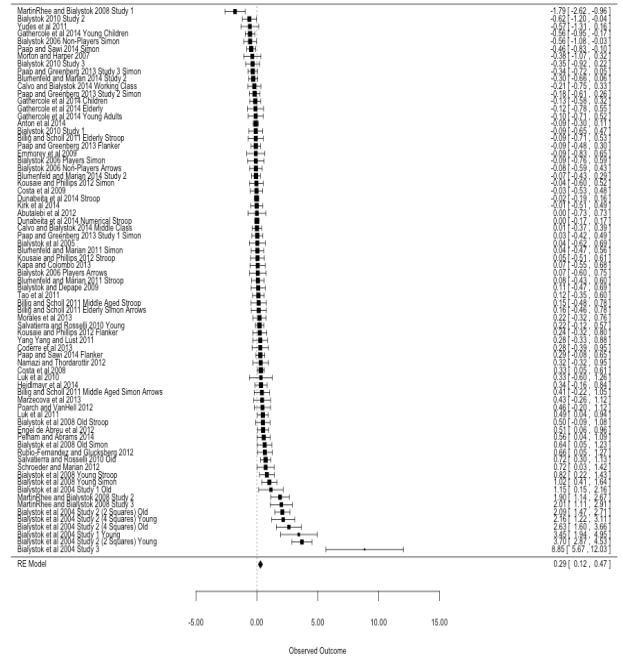
Figure 2: Forest Plot for Interference Costs
