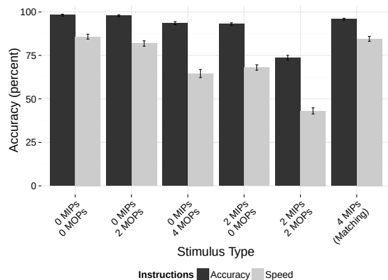
Figure 3: Accuracy across stimulus types split into Speed and Accuracy instruction conditions. Participants in the Speed instruction condition incorrectly classify the 2 MIPS 2 MOPS stimuli in which all of the colors matched between the two panels but two colors were not in the same positions. Error bars depict one standard error.
