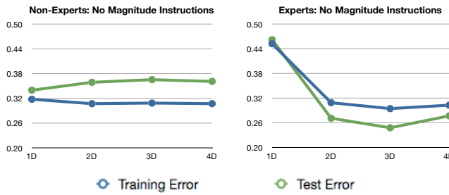
Figure 4 Error curves for non-metric MDS embeddings in Experiment 3
