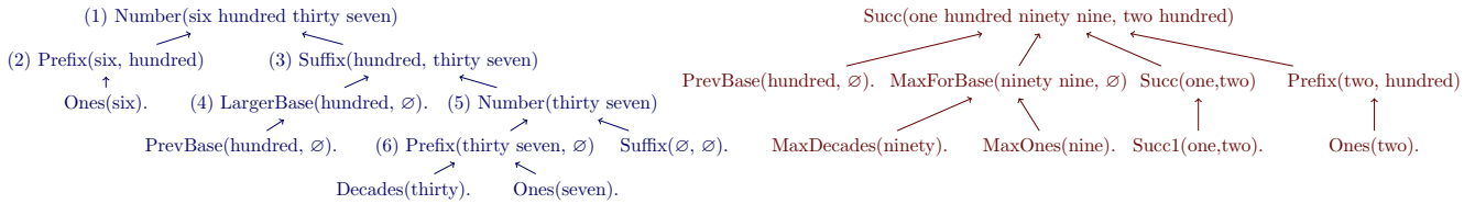
Figure 2: Example RCG parses for Number (Blue) and Succ (Red) relations.
