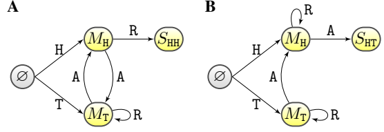
Figure 1: Markov chains for generating the first occurrence of the patterns HH (figure A) and HT (figure B). States S_{HH} and S_{HT} represent all sequences that end with the first occurrence of the expected pattern. States M_H and M_T represent all sequences that end with either an H or a T but do not contain the expected pattern. After the first transition out of the initial empty state ( \emptyset ), later transitions are characterized by either a repetition (R) or an alternation (A).
