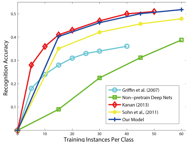
Figure 5: Mean per-class accuracy of Caltech-256 dataset as a function of number of training images. Griffin et al. (2007) provides baseline results. Deep convolutional neural networks do not perform well when trained solely on Caltech-256, because they overfit without additional training on significantly larger datasets, e.g., ImageNet (Zeiler & Fergus, 2014). Sohn et al. (2011) used features learned from a convolutional RBM. Kanan (2013a) used CSIFT features and multi-channel gnostic fields, and we achieved almost the same accuracy. Chance is 0.0039.
