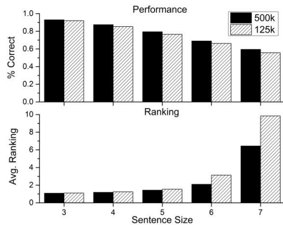
Figure 2. Performance from Figure 1 where m = 125,000 and results from a new simulation were m = 500,000 .
