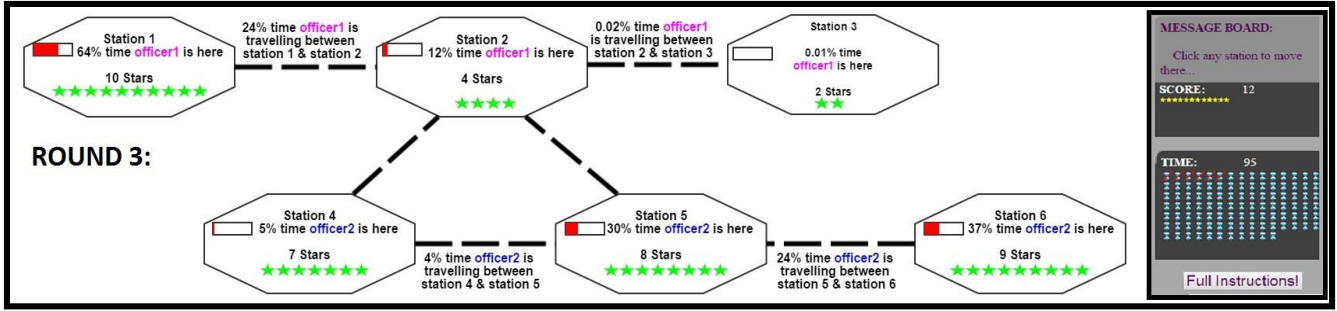
Figure 1. Game Interface
