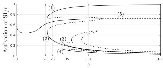
Figure 2: The bifurcation diagram. The solid and dashed lines indicate stable and unstable equilibria, respectively. Only the branches evolving to (1) [S_1 \text{ A B}] , (2) [S_2 \text{ A C}] , (3) [S_3 \text{ D B}] , (4) [S_4 \text{ D C}] , and (5) a blend of S_1 and S_2 are presented. The vertical lines indicate the \gamma values at each of which a disconnectivity graph was constructed (see Figure 3).
