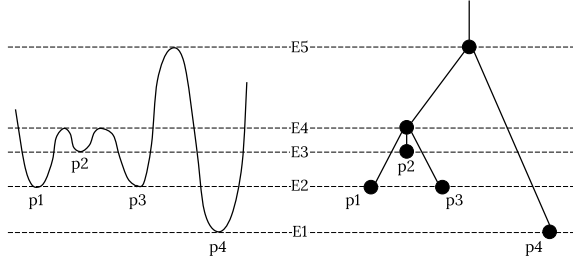
Figure 1: An arbitrary energy landscape (energy = -Total Harmony) and a disconnectivity graph constructed from the energy landscape. p1-p4 indicate the local minima and E1-E5 ( E1 < \dots < E5 ) indicate the energy levels.
