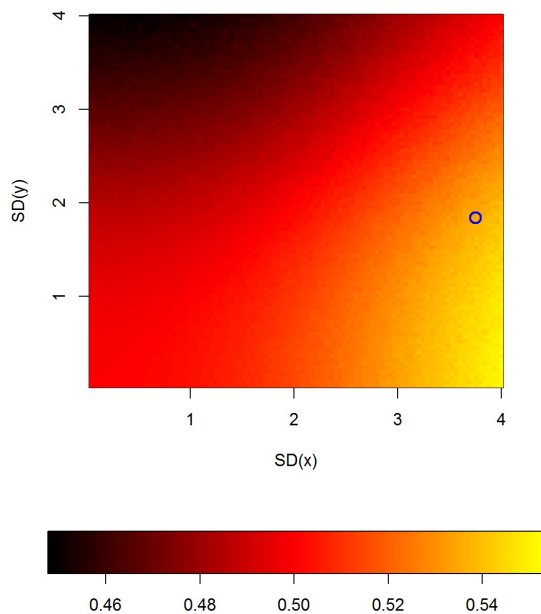
Figure 3: Simulated samples drawn from distributions with a common mean, Color indicates the mean proportion of the sum of the two samples that comes from the y sample
