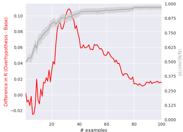
(b) Syntactic-semantic overhypotheses support rapid learning. The red line (left axis) plots the mean difference in R between runs of the overhypothesis model and runs of the base model as learning progresses. The gray line (right axis) tracks the average strength of the induced overhypothesis p(t = \text{color} \mid s = N/N) in the overhypothesis model. Shaded region represents bootstrapped 95% CI.
