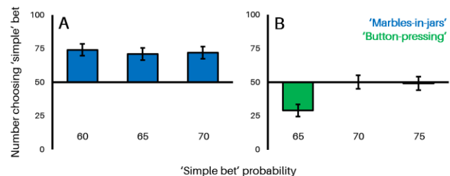
Figure 1. The number of participants who chose the ‘simple’ bet in (A) Experiment 1a and (B) Experiment 2a. The y-axis simply represents the number of participants (out of 100) who chose the simple bet (as opposed to the disjunctive bet). On the x-axis are the three different values of the simple bet for each experiment; note that these are not identical across experiments, by design. Error bars represent \pm 1 SE.
