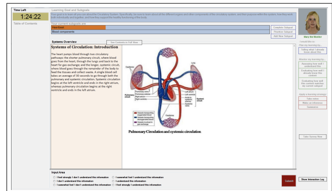
Figure 1: MetaTutor interface
