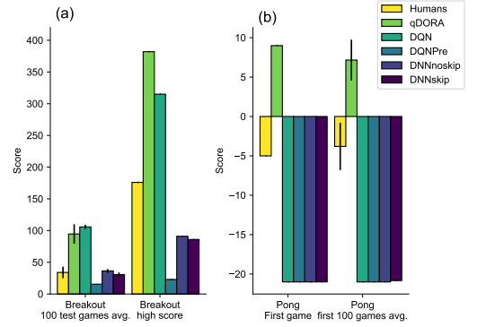
Figure 4: Game play performance for DORA and DNNs.
