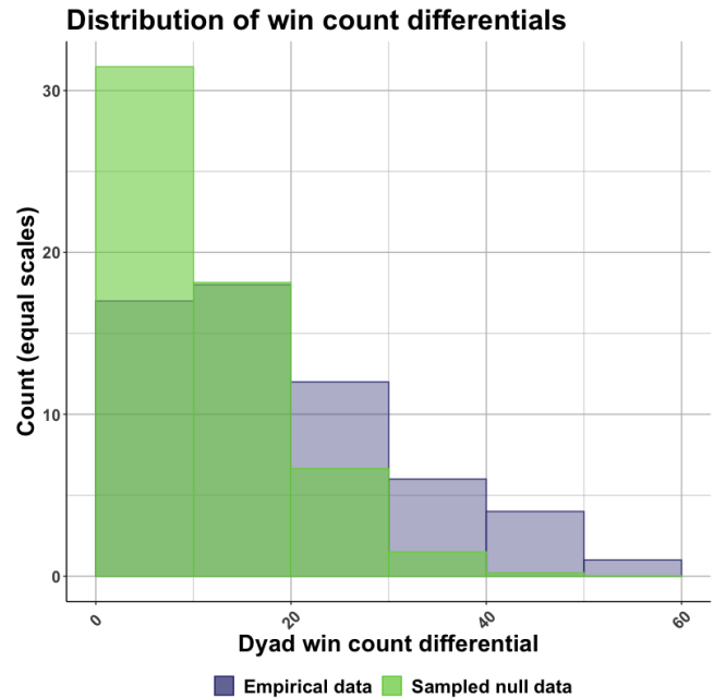
Figure 2: Empirical and null distributions of win count differentials within dyads. The null distribution is based on 10,000 samples but scaled to match the empirical counts. The empirical distribution has a heavier tail, suggesting that many players successfully exploited their opponents.
