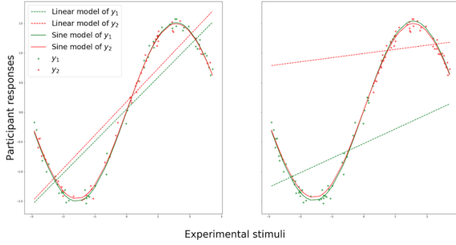
Figure 3: The sine and linear model fit to two different partitions of simulated data into y_1 and y_2 (the sine model is the data-generating model): a random partition (lefthand panel) and a partition based on the topographically distinct regions of the sine model’s contours (righthand panel). Both panels show the best-fitting parameterized versions of the sine and linear models, fit separately to each partition.
