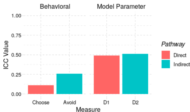
Fig. 7. A comparison of the Intraclass Correlation Coefficient (ICC) values of the behavioral measures (left) and the MAP estimates of the underlying model parameters (right) that index the function of the two pathways.
