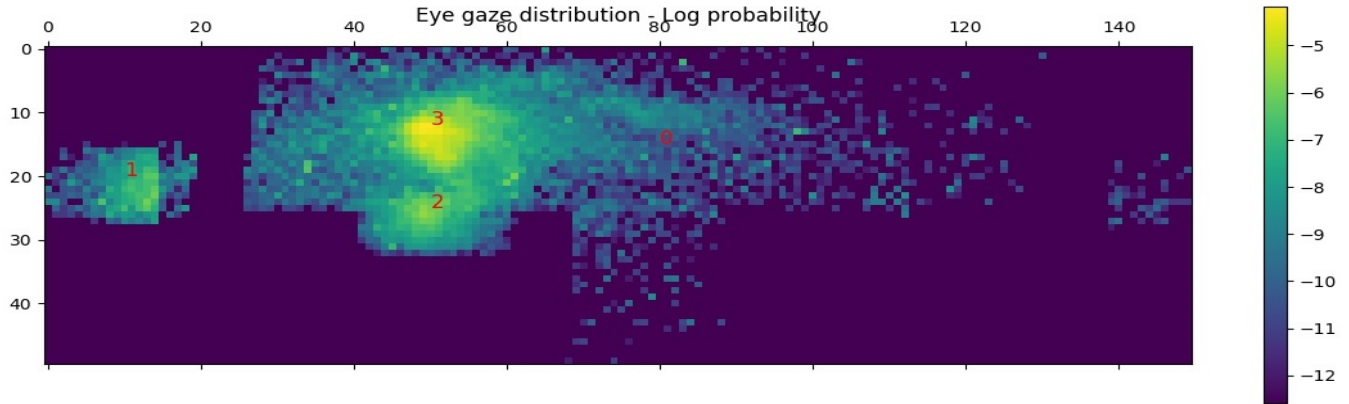
Figure 2: The figure presents the histogram of gaze intersection locations with objects in the field of view. The X and Y axes are the horizontal and vertical coordinates. Light colored areas are associated with areas with high probabilistic density. Three objects are marked by numbers in the figure. Objects 1 and 2 are the left mirror and the instrument cluster respectively. Object 3 is associated with the windshield, and the concentration of probability is linked to the focus on the road ahead.
