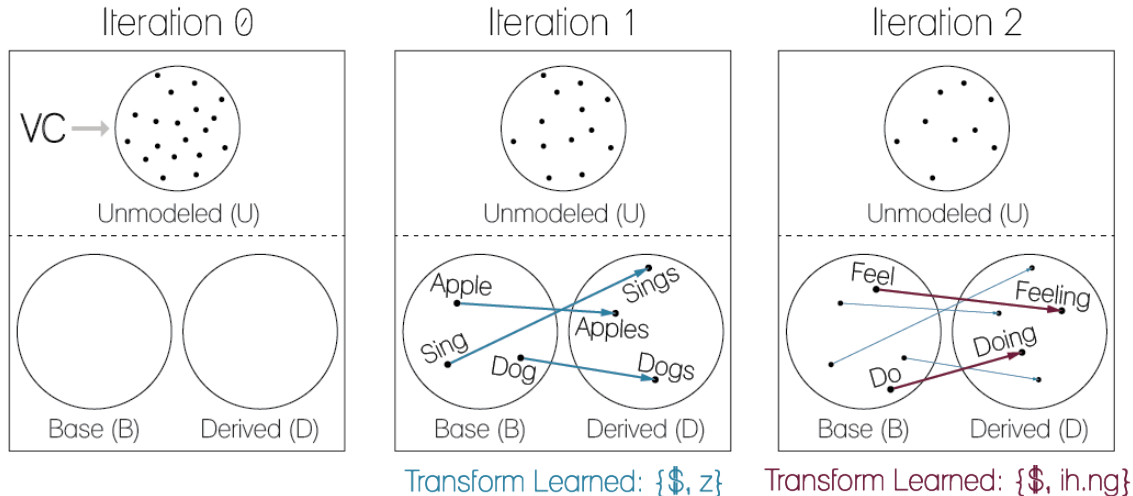
Figure 2: Overview of the algorithm. All wordpairs begin in the Unmodeled (U) set. A new transform is learned with each iteration, and the word forms it connects are moved into the Base (B) and Derived (D) sets.
