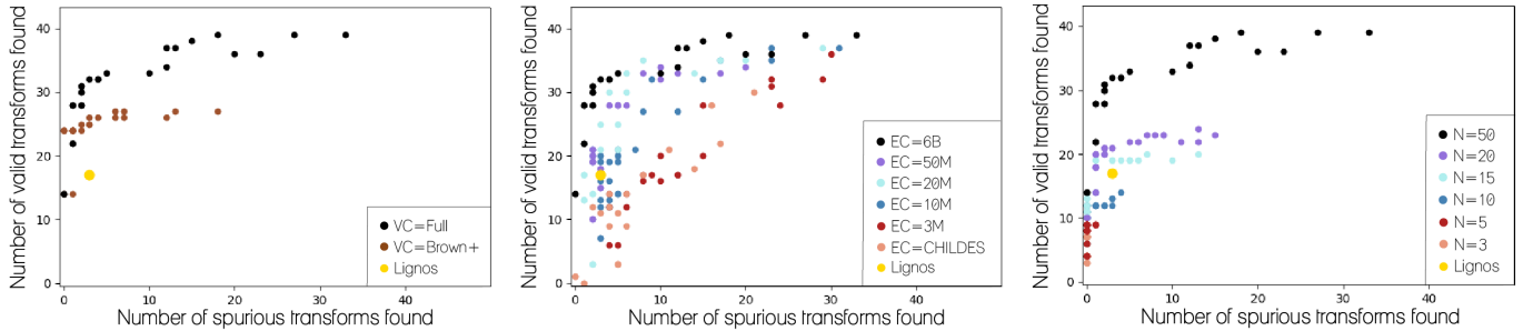
Figure 4: Trends in results for a low resource learner as a function of Vocabulary Corpus (left), Embedding Corpus (middle), or N (right), the number of suffixes considered in forming candidate transforms. We let T , L , W , and P vary within each color.
