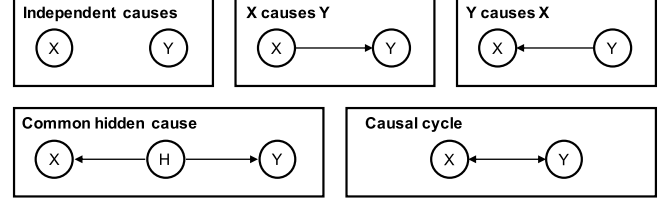
Figure 3: The causal structure hypotheses presented to participants.
