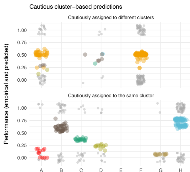
Figure 9. Predicted performance (colored) compared with actual performance (gray) for the cautious cluster-based approach.
