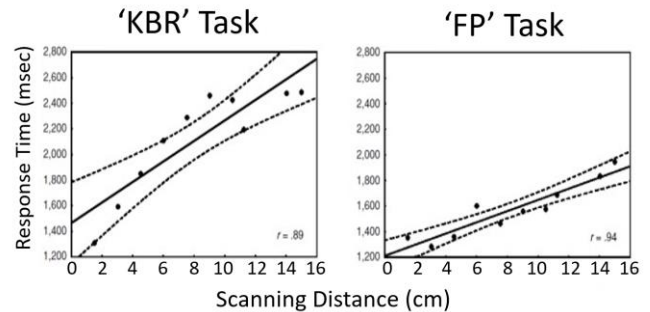
Figure 5: Comparison of linear relationships between scan time and distance between both original scanning tasks of Borst, Kosslyn and Denis (2006)
