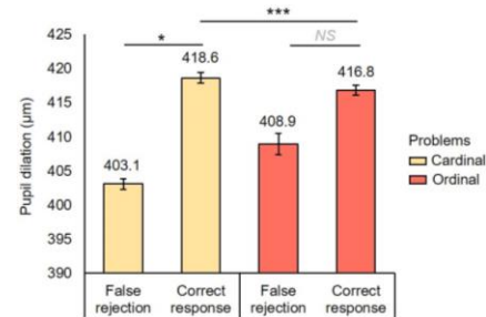
Figure 5: Pupil dilation on solvable problems. Error bars indicate upper margins of 95% confidence intervals.
