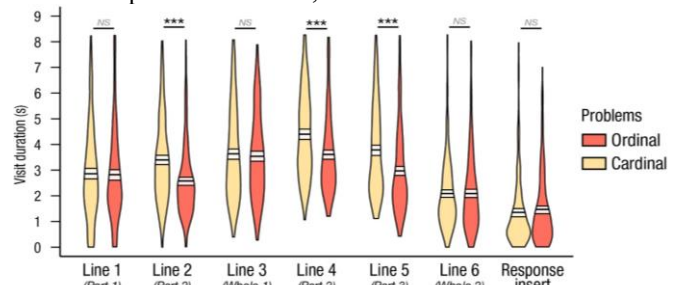
Figure 3: Visit duration per problem line
