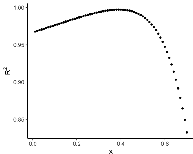
Figure 4: R^2 values between first-order word-word similarity and the weighted subtraction of third order space from second order space, as a function of x , the proportion of third order space subtracted from the second.
