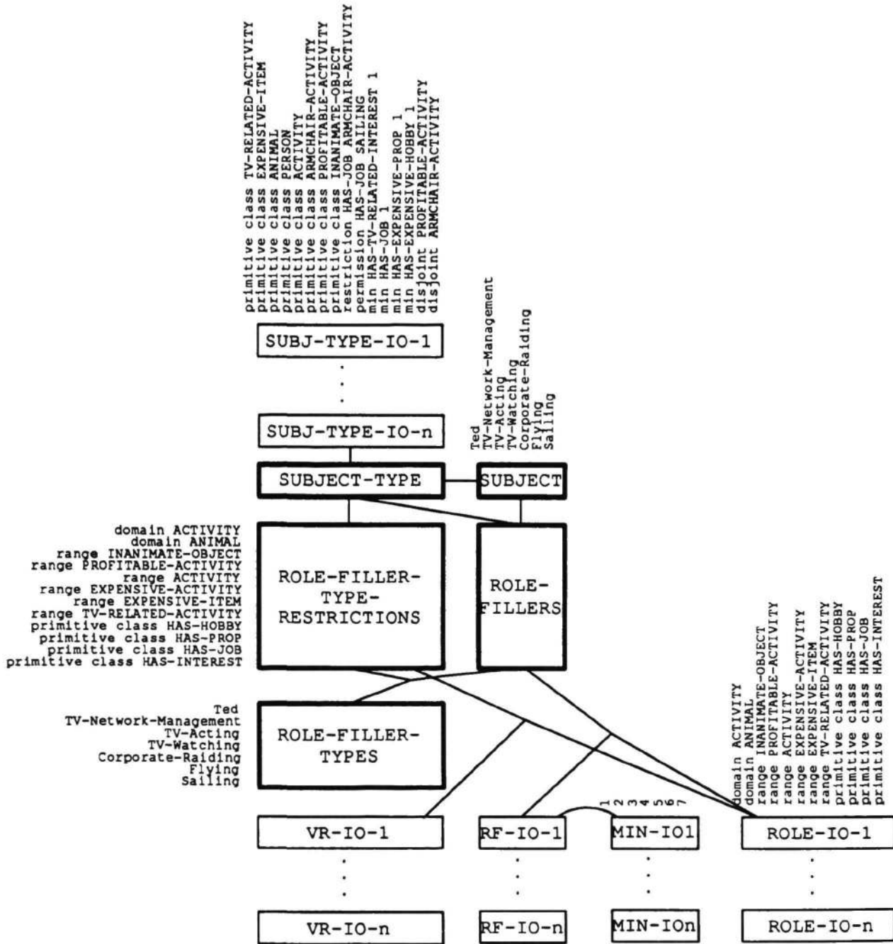
Figure 1: \mu KLONE has five important central modules (dark rectangles) and a variable number of subject-type, role, role-filler, minimum restriction, and value restriction IO modules. There are also auxiliary modules, which are not shown here. Those modules which directly constrain one another are connected. The meaning of each unit can be deduced from the printed descriptions. For modules with a single row of units, the meaning is the description in the unit's column. For modules with many rows, the meaning involves the conjunction of the descriptions in the row and column. For instance, the top left unit in the role-fillers module means that Ted is filling a role whose domain is ACTIVITY.
