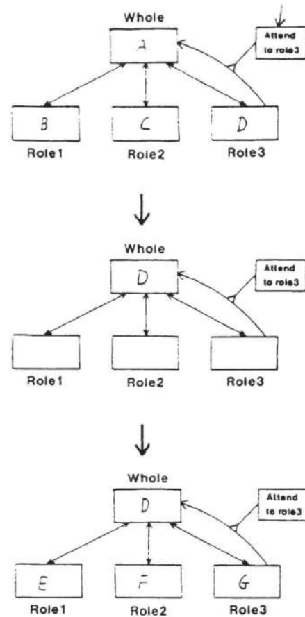
Figure 4: One way of using some additional hardware to allow the network to access the full description of node D from a role-specific reduced description. Even though the two descriptions correspond to quite different patterns of activity, their relationship should be non-arbitrary.
