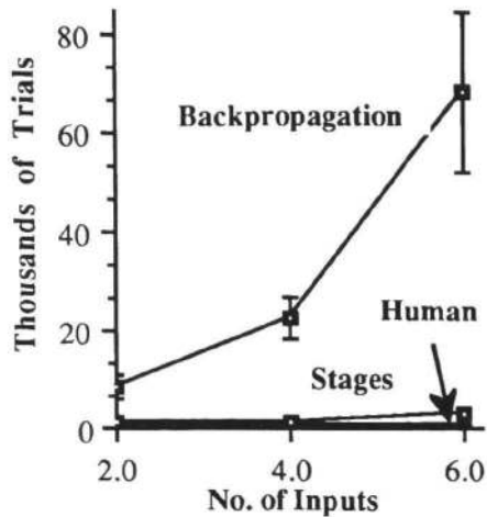
Figure 2. Trials to criterion for humans, backpropagation alone, and backpropagation with stages.
