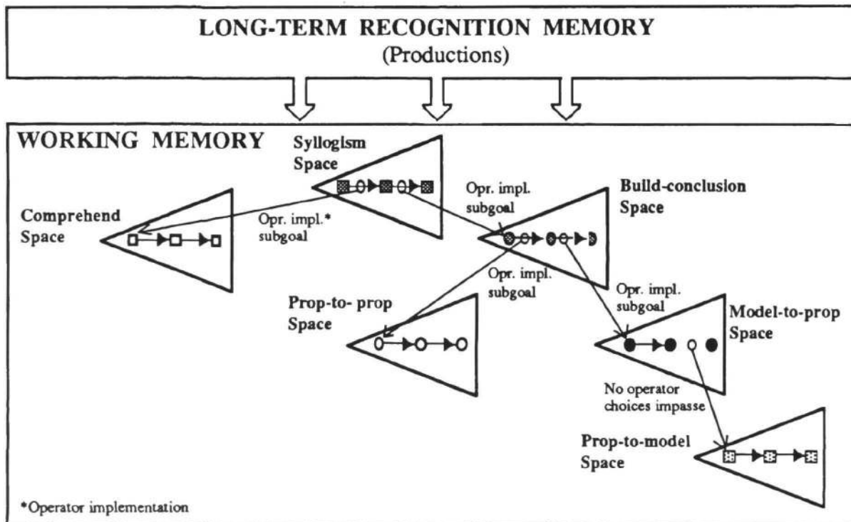
Figure 2: The structure of Soar.
