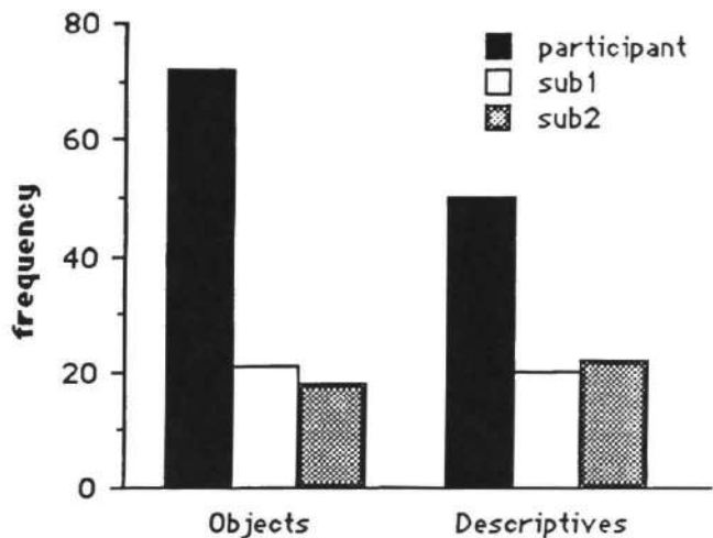
Figure 1: objects & descriptives
