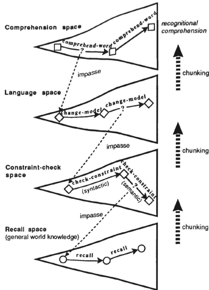
Figure 2: Achieving recognitional comprehension from deliberate comprehension in NL-Soar.
