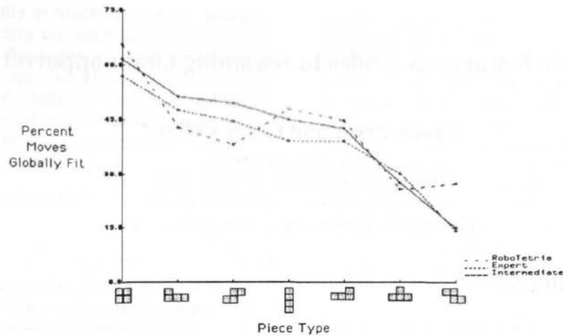
Figure 5: Global Fitness
