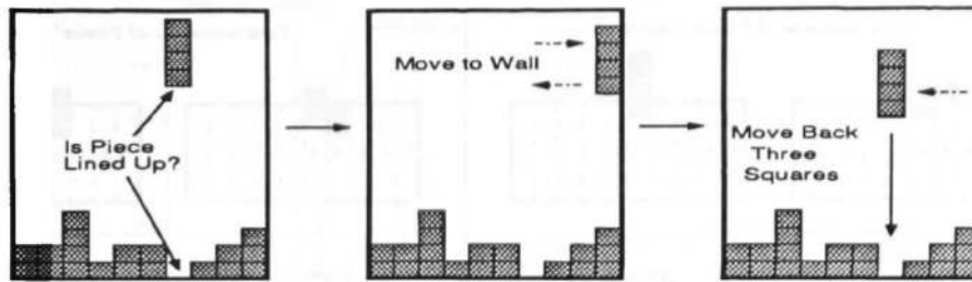
Figure 1: Translating for verification
