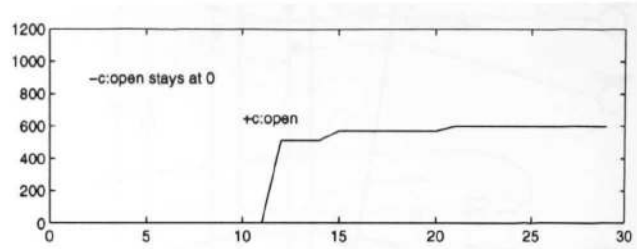
Figure 6: The activation trace for the query open(PO, Today)? ; where today is 20-Feb-95. The vertical axis denotes activation level and has a scale factor of 1000. The horizontal axis denotes number of simulation steps.
