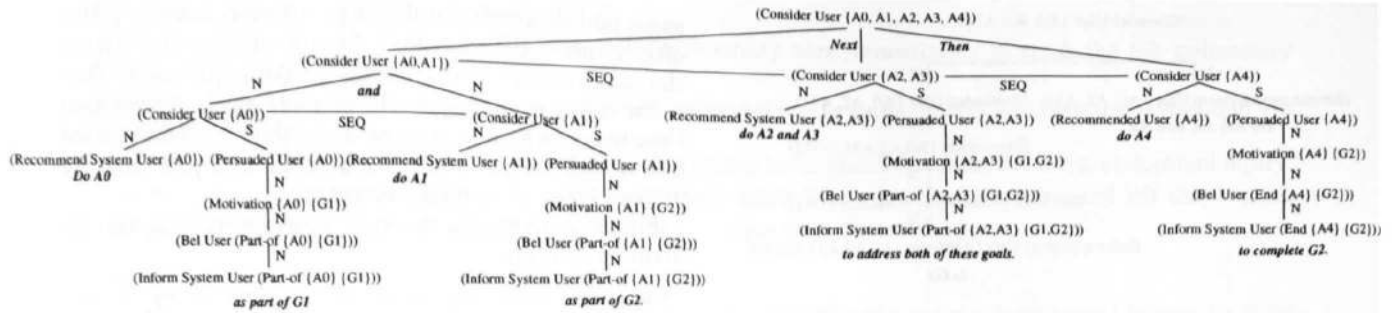
Figure 3: Text Plan for First Merged Message
