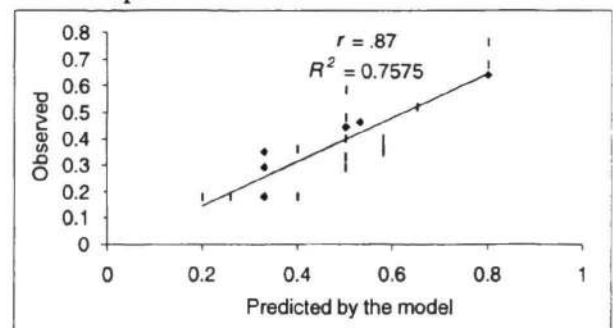
Figure 2: Predicted and observed probabilities across stimulus pattern conditions and age groups
