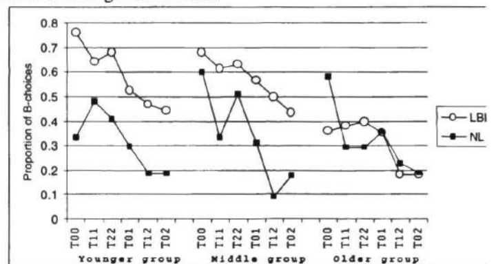
Figure 1: Proportions of B-choices by age and stimulus pattern condition.
