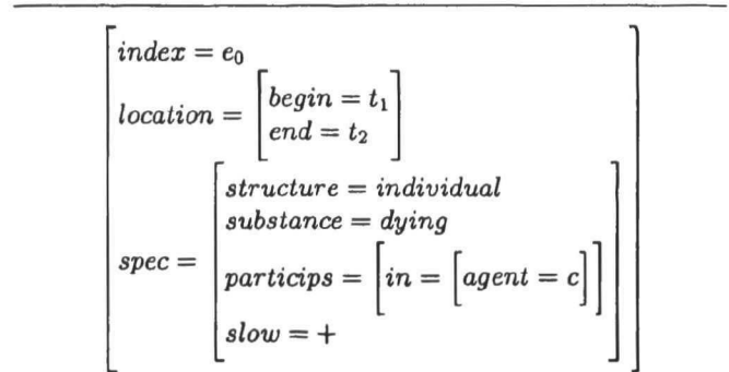
Figure 3: The KBE corresponding to Caesar dies slowly
