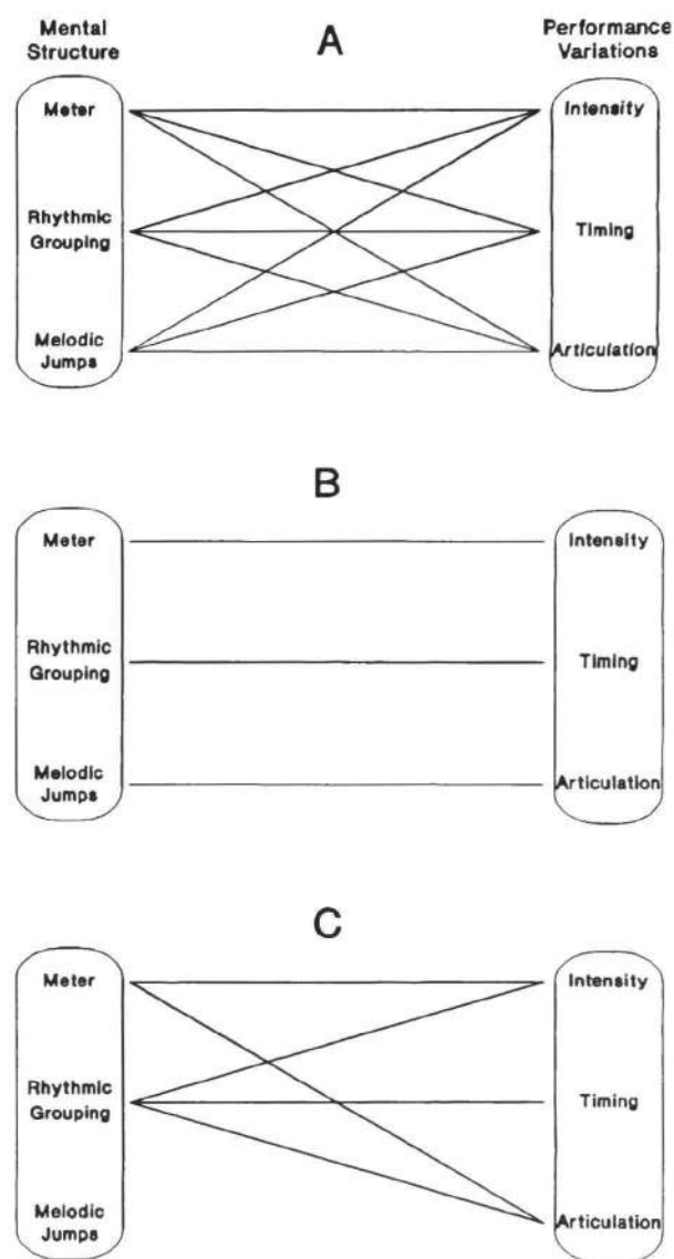
Figure 2. Three theoretical mappings of structure to expression.
