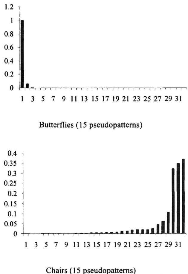
Figure 3. Hidden unit activation profile for Butterflies and Chairs in a network trained with 15 pseudopatterns.
