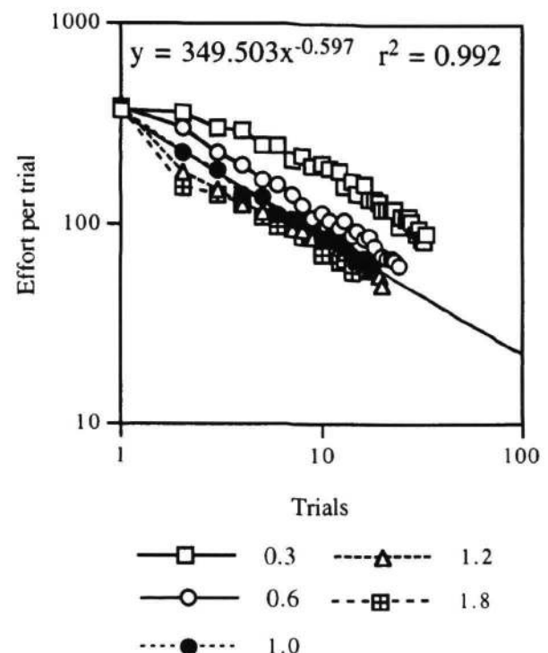
Figure 1: Learning curves for five different strengthening regimens in a cascading system, plotted with logarithmic coordinates. The straight line and the equation shows the power law fit for the sustained regimen ( pp = 1.0).
