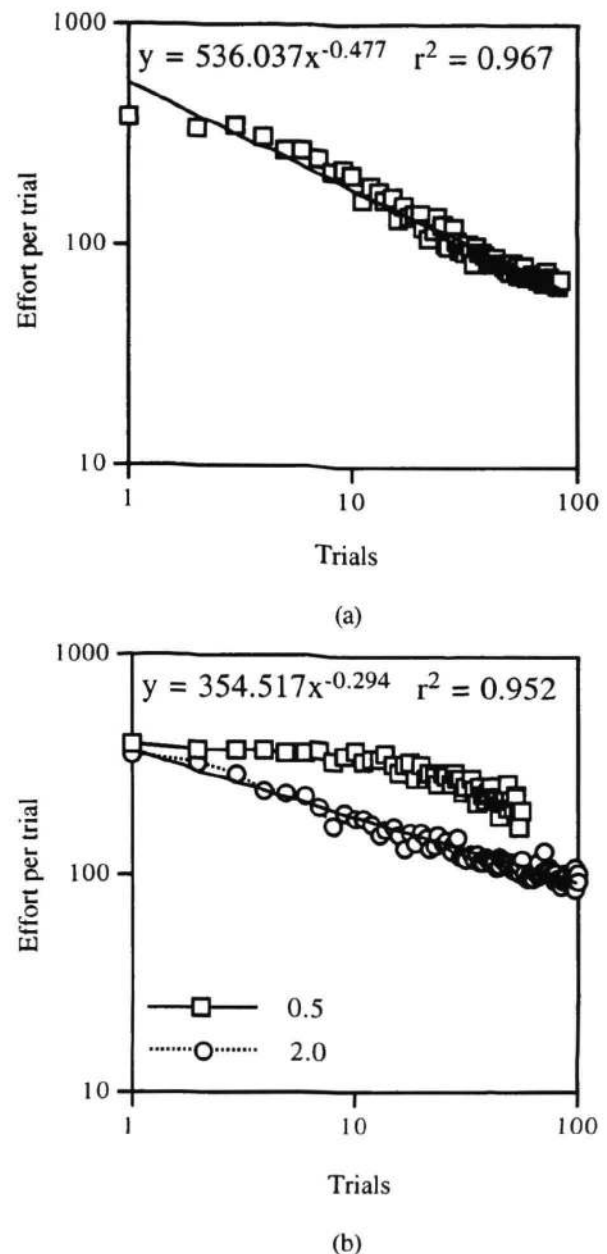
Figure 3: Learning curves for distributional regimens. Panel (a) displays the curve for a sustained regimen ( pp = 1.0 ), while panel (b) displays curves for dampened ( pp = 0.5 ) and amplified ( pp = 2.0 ) regimens.
