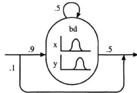
Figure 5: Centroid submodel for target bd .
