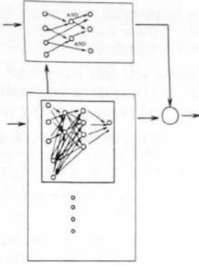
Figure 2: The implementation of CLARION.
