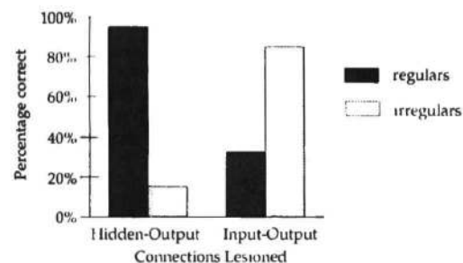
Figure 5: The effect of lesioning different pathways on the production of regular and irregular past tense classes.
