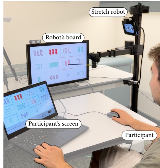
Figure 1: Experimental setup.
